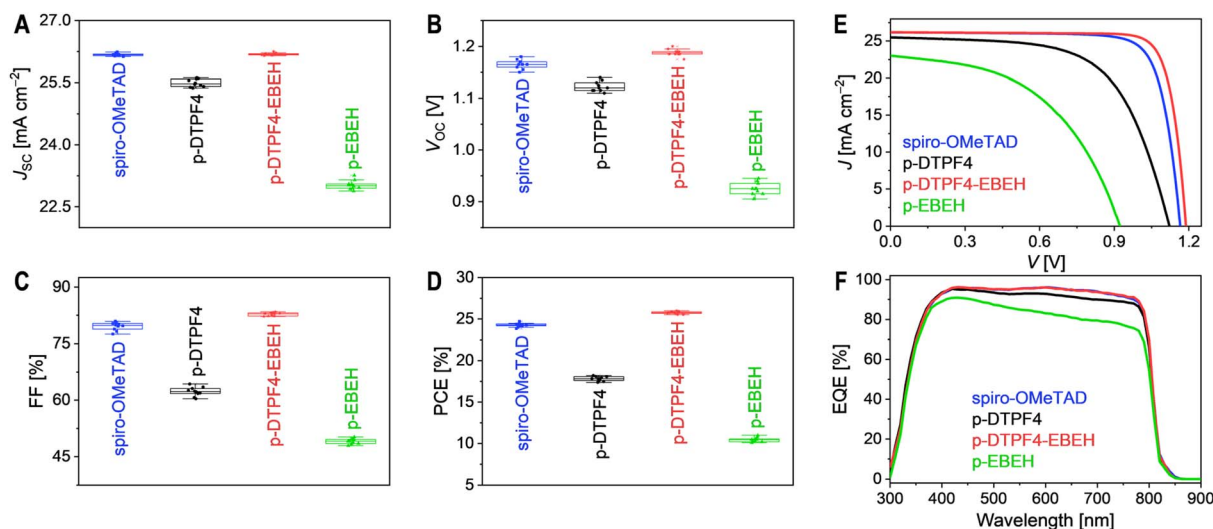
Fig. 3 (A–D) Statistical analysis of photovoltaic parameters of PSCs fabricated with varying hole transport layers under simulated AM1.5G irradiation at 100 mW cm -2 : (A) short-circuit photocurrent density ( J_{sc} ); (B) open-circuit voltage ( V_{oc} ); (C) fill factor (FF); (D) power conversion efficiency (PCE). (E) Representative photocurrent density–voltage ( J – V ) curves. (F) External quantum efficiency (EQE) spectra.
