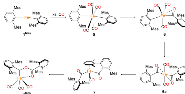
Scheme 2 Proposed reaction pathway for formation of 4^{\text{Mes}} from 1^{\text{Mes}} . Note that 6a has only been observed spectroscopically in solution, all other species have been isolated and characterised by single crystal X-ray diffraction (See Section 2.3).
