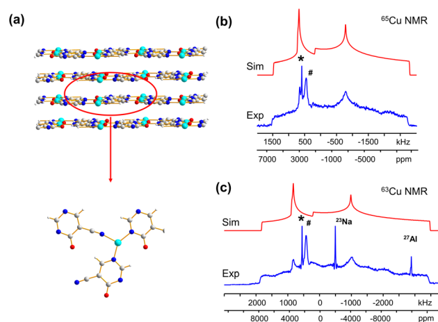
Fig. 6 (a) The long-range and local structure of \text{Cu}_3(4\text{hyppymca})_3 . The experimental (blue) and simulated (red) ^{65}\text{Cu} static NMR spectra and ^{63}\text{Cu} static NMR spectra at 21.1 T are shown in (b and c), respectively. ^{27}\text{Al} marks a signal from probe background. The signal from ^{23}\text{Na} background is also marked in the ^{63}\text{Cu} NMR spectrum, but is truncated for clarity.
