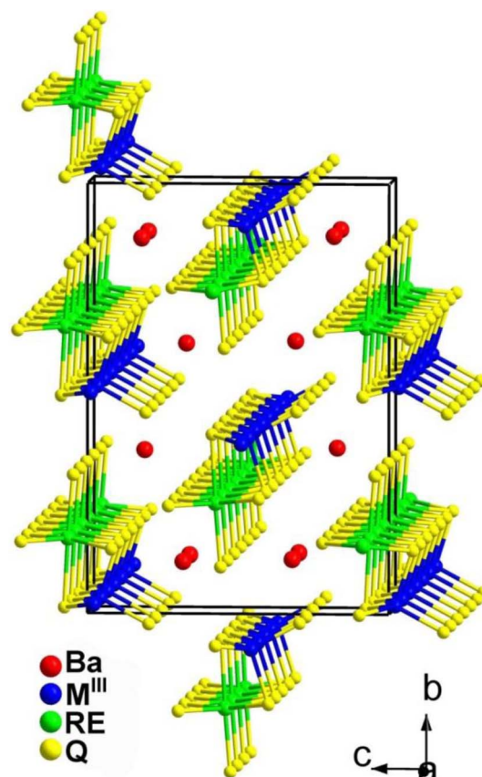
Fig. 7 Structure of Ba_2REM^{III}Q_5 along the bc plane with the unit cell outlined.
