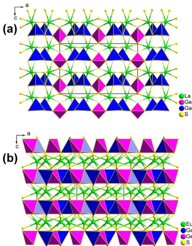
Fig. 6 Structures of (a) La_2Ga_2GeS_8 and (b) Eu_2Ga_2GeS_7 along the ac plane with the unit cell outlined.
