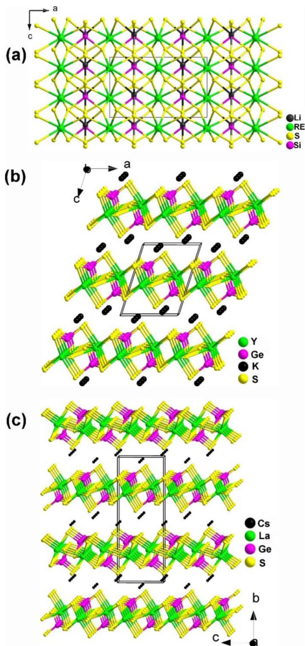
Fig. 11 Structures of (a) \text{LiRESiS}_4 (space group: \text{Ama2} ), (b) \text{KYGeS}_4 (space group: P2_1 ), and (c) \text{CsLaGeS}_4 (space group: P2_12_12_1 ) with the unit cell outlined.
