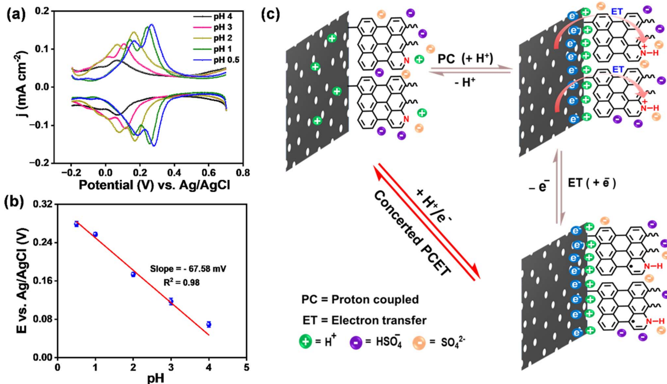
Fig. 6 Understanding the capacitance enhancement in the light of proton-coupled electron transfer mechanism. (a) DPV of the ANT/GR electrode recorded with varying pH of H_2SO_4 solution using 0.1 M KCl as electrolyte. (b) Reduction potential vs. pH plot (from DPV data). (c) Schematic illustration of interfacial PCET pathway to and from different nitrogens present in the ANT/GR electrode.
