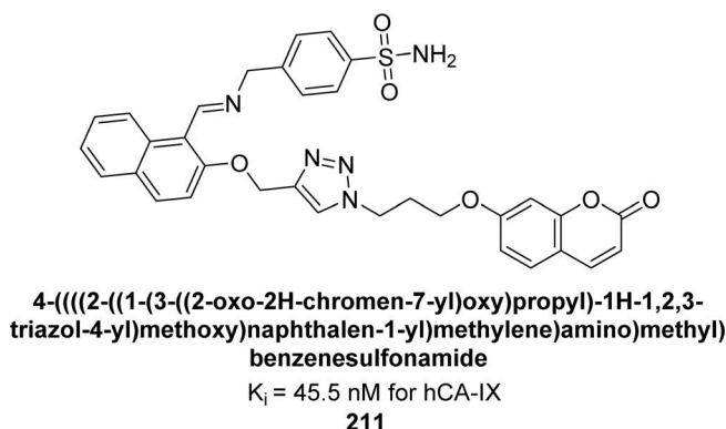
Fig. 76 Chemical structure of compound 211 ; its K_i value against hCA-IX along with docking image of compound 211 .
