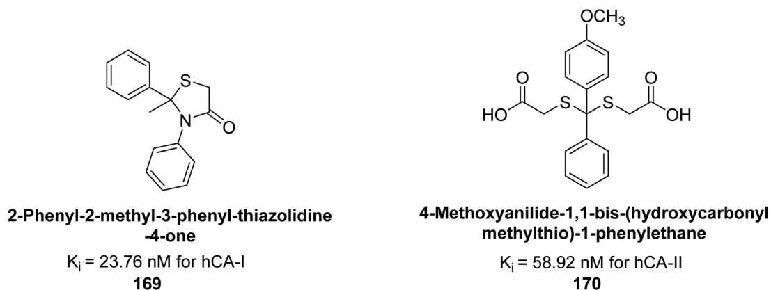
Fig. 58 Chemical structures of compounds 169 and 170 and their K_i values against hCA-I & II.
