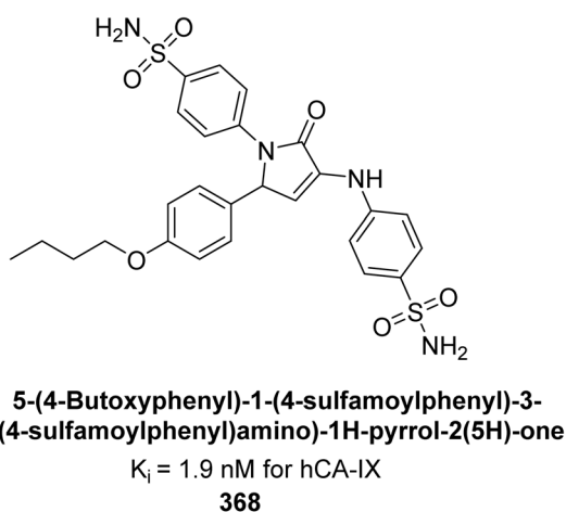
Fig. 131 Chemical structures of compounds 367 and 368 ; their K_i values against hCA-I and IX along with their docking images.
