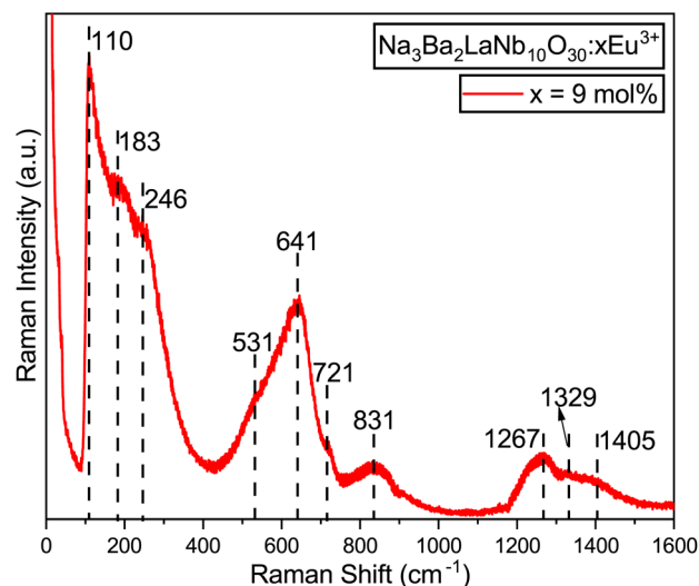
Fig. 10 Raman spectrum of the \text{Na}_3\text{Ba}_2\text{LaNb}_{10}\text{O}_{30}:\text{xEu}^{3+} ( x = 9 \text{ mol\%} ) phosphor at room temperature.
