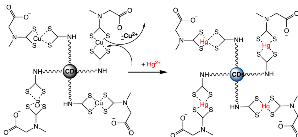
Scheme 7 Fluorescent "Turn On" nanosensor for surface-bound \text{CuDTC2} complex \text{Hg}(\text{II}) detection based on \text{Cu}(\text{II}) displacement due to \text{Hg}(\text{II}) .
