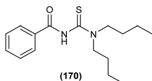
Fig. 95 Structure of N -benzoyl- N' , N' -dibutyl thiourea.
