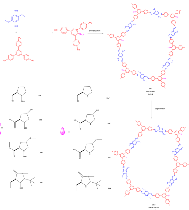
(Asymmetric \alpha -aminoxygation Reaction)
