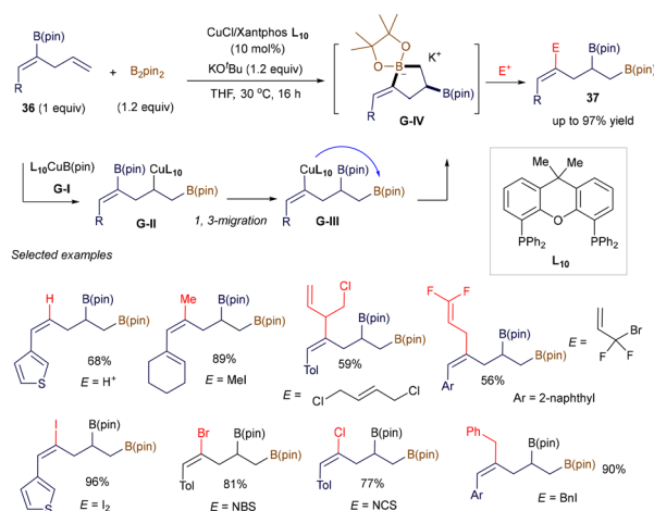
Scheme 11 Boron-copper 1,3-rearrangement.
