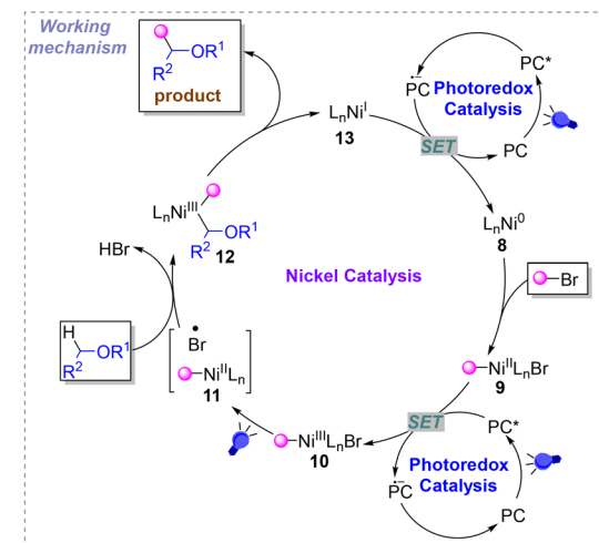
Scheme 5 \text{Csp}^3\text{-Csp}^3 cross-coupling reaction of alkyl bromides with ethers (Paixão and König's work).
