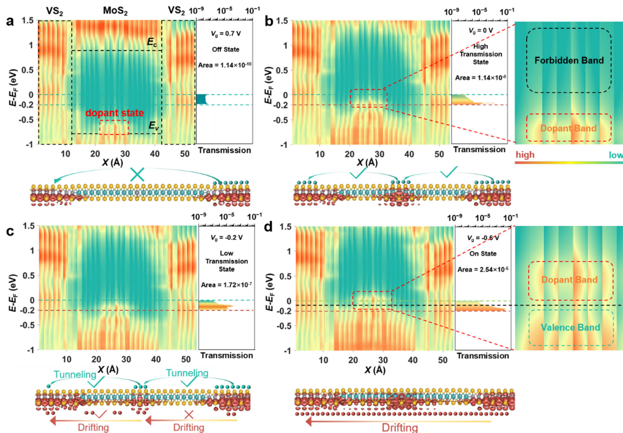
Fig. 4 PDOS profiles, electron transmission spectra, and real-space DOS at -0.2 eV of a V-MoS 2 transistor, with L_{ch} = 3.0 nm and V_{sd} = 0.2 V, calculated under different gate voltages ( V_g ) of 0.7 V (a), 0 V (b), -0.2 V (c), and -0.6 V (d). Insets on the right of (b) and (d) show magnified views of the forbidden band, the dopant band, and the valence band in the PDOS profiles. The orange arrows (balls) indicate drift transport (holes), while the cyan arrows (balls) denote tunneling transport (holes).
