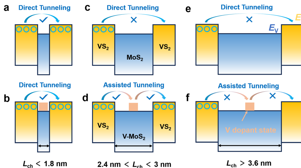
Fig. 5 Schematic illustration on the electronic functionalities of the V-doped states at different channel lengths. Band diagrams of MoS 2 and V-MoS 2 at L_{ch} < 1.8 nm (a, b), 2.4 nm < L_{ch} < 3.0 nm (c, d) and L_{ch} > 3.6 nm (e) and (f) are plotted. The blue hollow circles represent holes. The yellow and blue regions signify the VS 2 electrodes and the MoS 2 channel, respectively. The orange regions represent the V-doped states at the top of the MoS 2 valence band.
