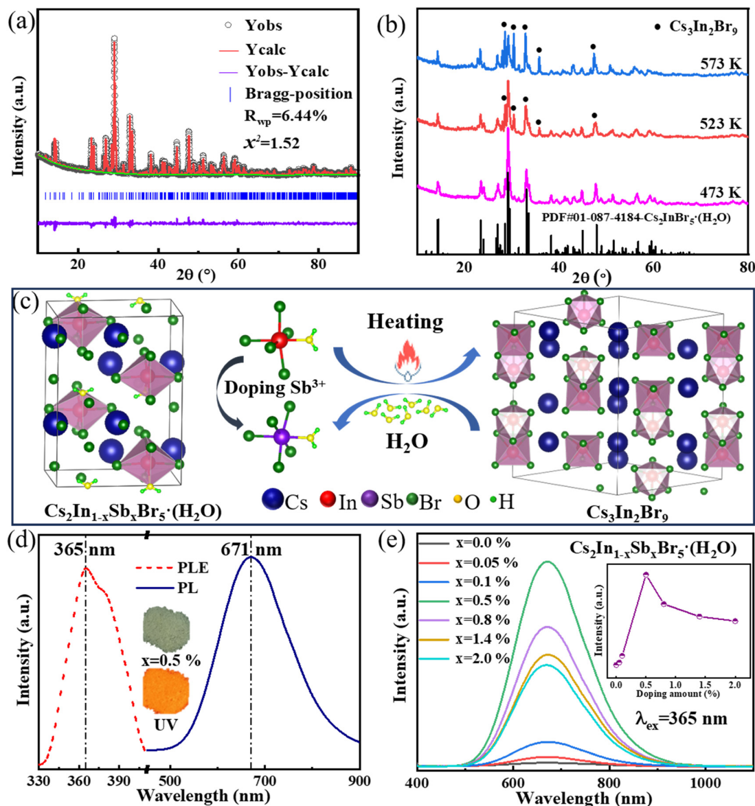
Fig. 2 (a) Rietveld refinement results of Cs 2 InBr 5 (H 2 O) samples; (b) XRD patterns after annealing at different temperatures; (c) schematic representation of the reversible transformation between Cs 2 InBr 5 (H 2 O) and Cs 3 In 2 Br 9 crystal structures; (d) excitation (red line) and emission (blue line) spectra of Cs 2 InBr 5 (H 2 O):Sb 3+ (inset: photograph of the 0.5% Sb 3+ sample under ambient light and 365 nm UV light); (e) photoluminescence spectra of Cs 2 In 1-x Sb x Br 5 (H 2 O) ( x = 0-2.0\% ), the inset shows the changes in Sb 3+ doping concentration and PL intensity.
