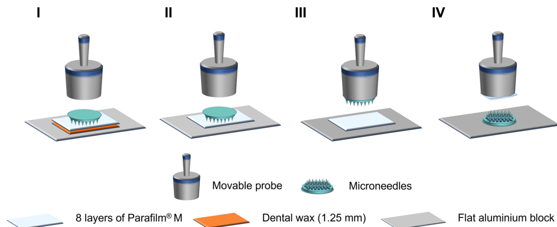
Fig. 2 Different experimental configurations for MN Paraform® M insertion study with setup I, II, III and IV.
