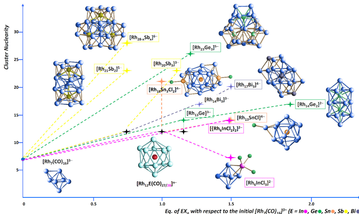
Fig. 9 Growth trend of heterometallic carbonyl clusters for the various Rh-E systems as a function of the added equivalents of EX_n ( X = Cl, Br ; n = 2-4 ). Carbonyl ligands have been omitted in the stated formulas, for sake of clarity. Rh atoms are depicted in blue, in magenta, Ge in bright green, Sn in orange, Sb in yellow, Bi in violet.
