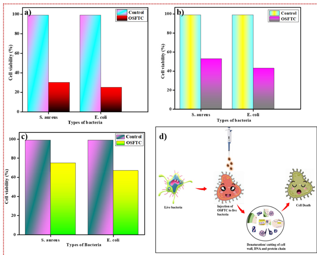
Fig. 7 (a–c) Cell viability percentage for 100 \mu\text{L} , 200 \mu\text{L} , and 300 \mu\text{L} of 20.3 \times 10^{-2} \text{ M} solution of OSFTC, (d) mechanism for killing bacterial cells via ROS species.
