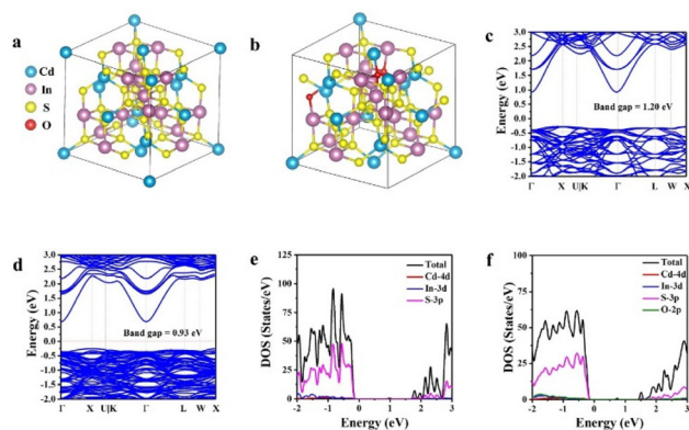
Fig. 6 Side view of (a) bulk CdIn 2 S 4 and (b) bulk CdIn 2 S 4 with three S atoms replaced by O atoms. Band structure of (c) CIS and (d) OCIS. Density of states of (e) CIS and (f) OCIS.
