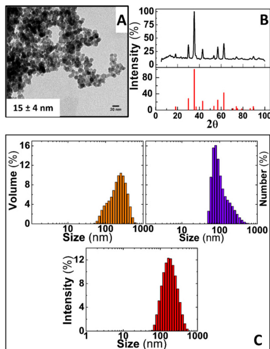
Fig. 2 Physico-chemical characterisation of iron oxide nanoparticles. (A) Representative TEM image of sucrose coated IONPs. (B) XRD diffraction pattern of IONPs performed in dried powders, iron oxide COD: 96-900-9769 (C) DLS diagrams of IONPs dispersed in ddH 2 O and weighted by volume (orange columns), number (purple columns) and intensity (red columns). Scale bar in (A) = 20 nm.
