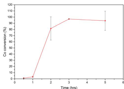
Fig. 11 Co conversion rate as a function of milling time. Milling conditions: 500 rpm, 3 g of powder (Al + LCO), n_{\text{Al}}/n_{\text{Co}} = 1.0 , P/B = 0.15, 7 \times 10 mm balls. These results report the average of 3 experiments performed in the same conditions.
