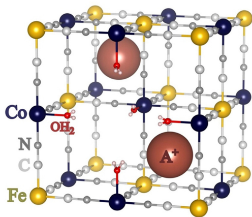
Fig. 1 Scheme of one unit cell of the A_2Co_4[Fe(CN)_6]_{3.3}\square_{0.7-n}OH_2 PBAs (brown balls stand for alkali cations, blue for Co ions, yellow for Fe ions, light grey for carbon atoms, dark grey for nitrogen atoms, and red for oxygen atoms). Zeolitic water molecules are omitted for clarity.
