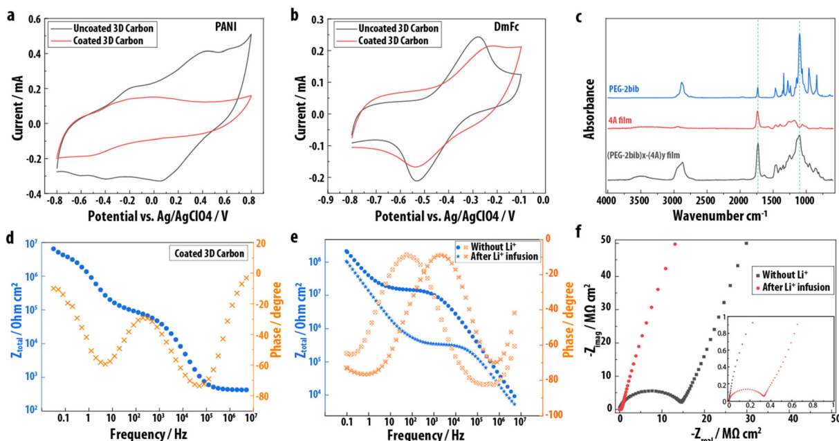
Fig. 3 (a and b) CVs of PANI (a) and DmFc (b) before and after electrodeposition on 3-D carbon. (c) ATR-FTIR spectra of PEG-2bib (blue), an electro-polymerized 4A film (red), and an EPoN-derived (\text{PEG-2bib})_x-(4\text{A})_y films (black). Dashed lines indicate position of carbonyl ( 1730\text{ cm}^{-1} ) and ether ( 1100\text{ cm}^{-1} ) absorption bands. Spectra are shifted vertically for clarity. (d) Bode plot of the solid-state EIS on the top surface of a 3-D carbon coated with a (\text{PEG-2bib})_x-(4\text{A})_y thin film. (e and f) EIS spectra of (\text{PEG-2bib})_x-(4\text{A})_y films on a planar gold substrate before and after lithium infusion: (e) Bode plot, (f) Nyquist plot.
