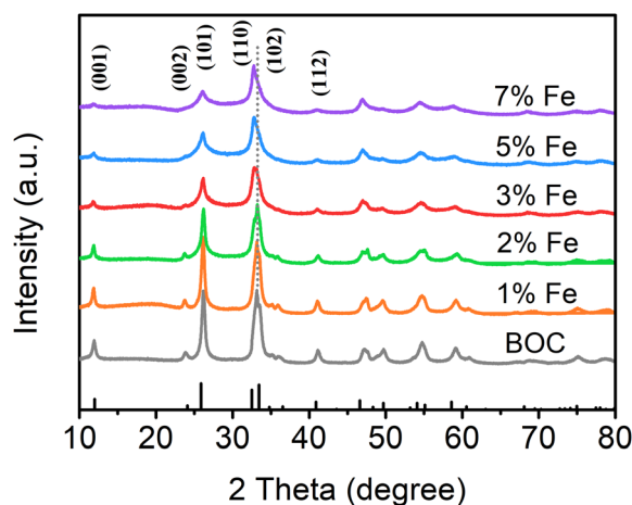
Fig. 1 XRD patterns of samples with different Fe doping amounts, BOC, 1% Fe-BOC, 2% Fe-BOC, 3% Fe-BOC, 5% Fe-BOC, and 7% Fe-BOC.
