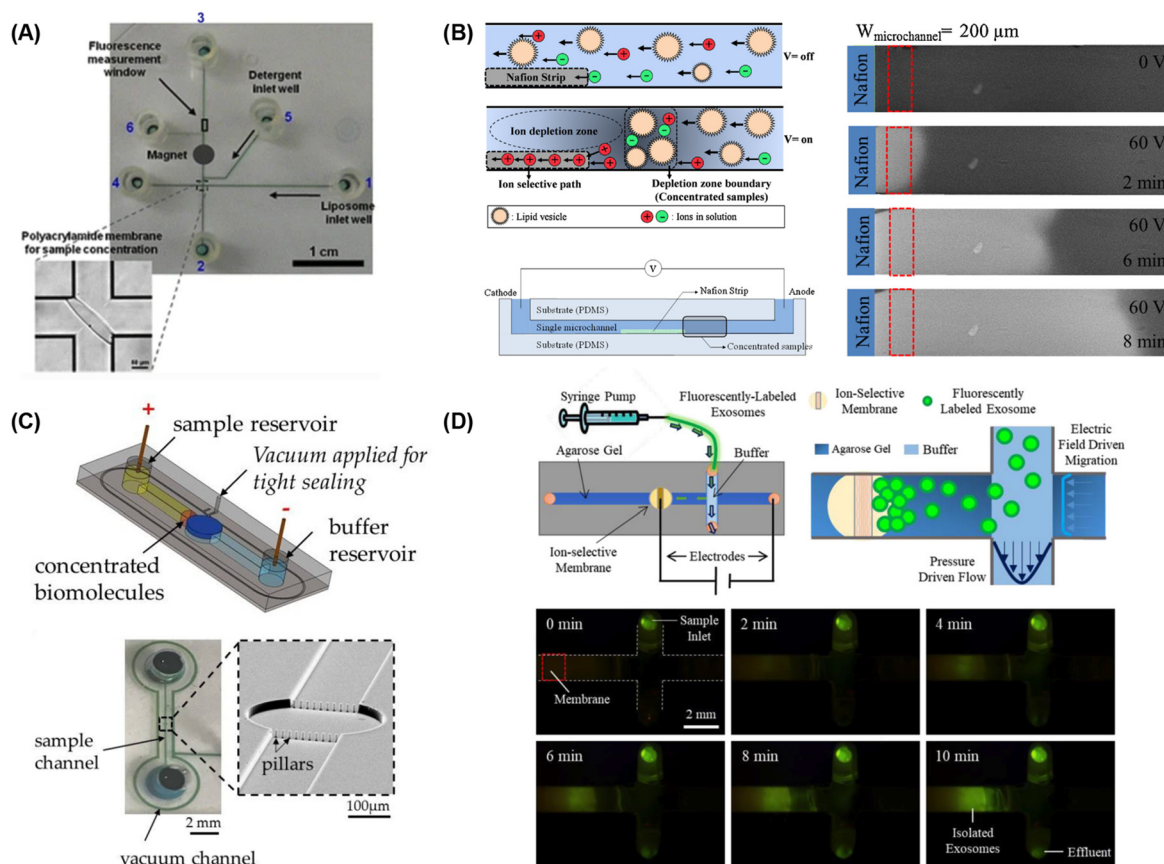
Fig. 5 Microfluidic lipid vesicle concentration techniques. (A) Electrostatic concentration of liposomes against a photolithographically-patterned polyacrylamide gel membrane (reproduced from ref. 222 with permission from Springer, copyright 2011). Liposome concentration via microfluidic ion concentration polarization utilizing (B) a Nafion membrane patterned on a microchannel floor (reproduced from ref. 223 with permission from Elsevier, copyright 2016), (C) conductive nanoporous polymer deposited in a sealed chamber (reproduced from ref. 224 with permission from MDPI, copyright 2018), and (D) capture of nanoparticles at the surface of an ion-selective membrane during continuous sample perfusion (reproduced from ref. 225 with permission from Wiley, copyright 2018).
