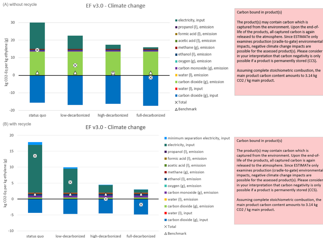
Fig. 5 Climate Change Impact of laboratory-scale electrochemical \text{CO}_2 reduction to ethylene in the ESTIMATE tool. (A) Without recycle of unreacted \text{CO}_2 , (B) including a recycle of unreacted \text{CO}_2 . Note the different scales of the y-axes. The different bars correspond to the different background system scenarios defined in section 2.4.
