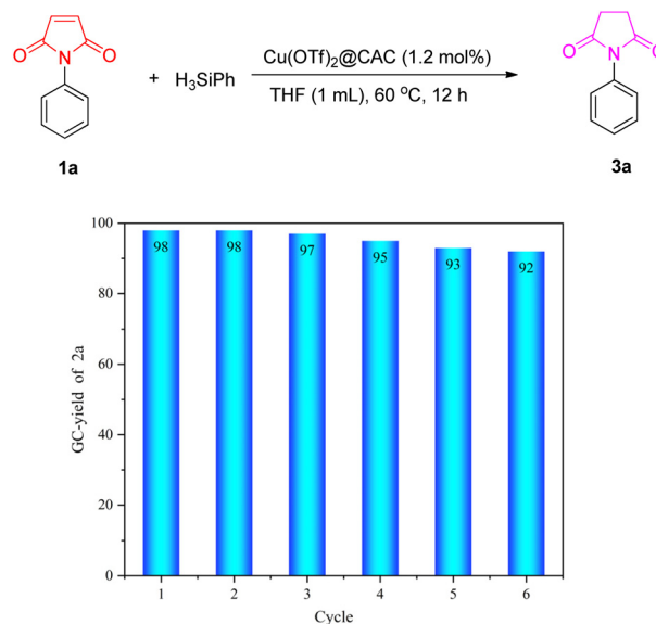
Fig. 5 Reuse of the \text{Cu}(\text{OTf})_2\text{@CAC} .
