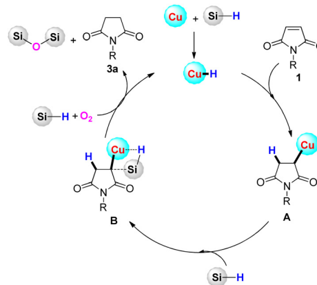
Scheme 3 Proposed mechanism for the \text{Cu}(\text{OTf})_2\text{@CAC} -catalyzed selective reduction of maleimides.
