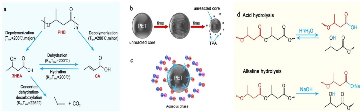
Fig. 4 (a) Proposed reaction network for PHB-to-propylene conversion, 43 (b) proposed shrinking-core model for the hydrolysis of PET over Brønsted acids, 120 (c) hydrolysis mechanism over alkaline catalysts and surfactants, 115 and (d) the hydrolysis mechanism in acid and alkaline solutions. 43
