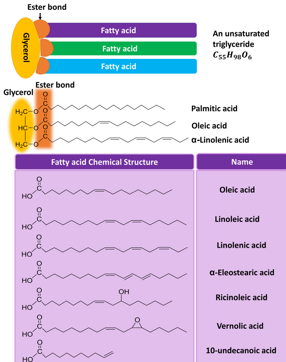
Fig. 6 (Top) Example of an unsaturated triglyceride in vegetable oils, which is composed of glycerol and fatty acids (figure on the top is redrawn from ref. 69 with kind permission of the website owner). (Bottom) Chemical structure of some common fatty acids (figure on the bottom is redrawn by the authors in ChemDraw from ref. 70 with kind permission from RSC, copyright 2010).
