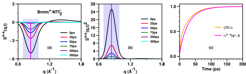
Fig. 5 For \text{Bmim}^+/\text{NTf}_2^- at 400 K and computed from molecular dynamics simulations described in reference 20, (a) the cation head-anion subcomponent S^{H-A}(q, t) , (b) its value squared, S^{H-A}(q, t)^2 , and (c) a comparison between \alpha^{H-A}(q^*, t) and \zeta(t)/\mu where q^* is taken as the wavenumber for charge alternation. The location of q^* is denoted with a vertical purple line in subfigures (a) and (b) and the whole charge alternation regions with a translucent magenta box. Notice how similar the relaxations of \alpha^{H-A}(q^*, t) and \zeta(t)/\mu are. In our different studies we consistently find that the relaxation of \zeta(t)/\mu tends to fall somewhere between that of the adjacency feature and that of the slowest (smallest q ) relevant intermolecular mode; depending on the length of alkyl tails, this can be the charge alternation feature or the prepeak.
