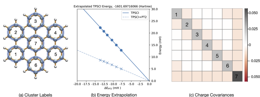
Fig. 7 Hexabenzocoronene. (a) Molecular structure and cluster indices. Active space (42e, 42o) includes all \pi orbitals. (b) Extrapolation of the energy of the singlet ground state. Units of milli-Hartree. (c) Charge covariance matrix, \text{cov}(\hat{N}_i, \hat{N}_j) .
