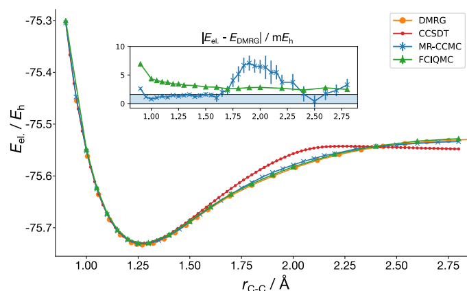
Fig. 6 The binding curve of the 1\Sigma_g^+ state of C_2/cc\text{-pVDZ} in the range of 0.9-2.8 \text{\AA} separation. All-electron MR-CCMCS calculations are based on CASSCF orbitals and use an (8e, 8o) CAS as a reference space, with clusters truncated at the double excitation level from this. The FCIQMC data is from Ref. 39, and the DMRG data is from 33, and the CCSDT data is from the ccpy package developed by Piecuch and coworkers. 40 The inset shows the error in the MR-CCMC and FCIQMC energy relative to DMRG.
