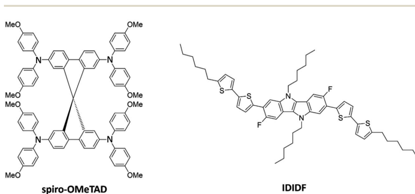
Fig. 1 Chemical structure of spiro-OMeTAD and the indolo[3,2- b ]indole-based IDIF hole-transporting materials.
