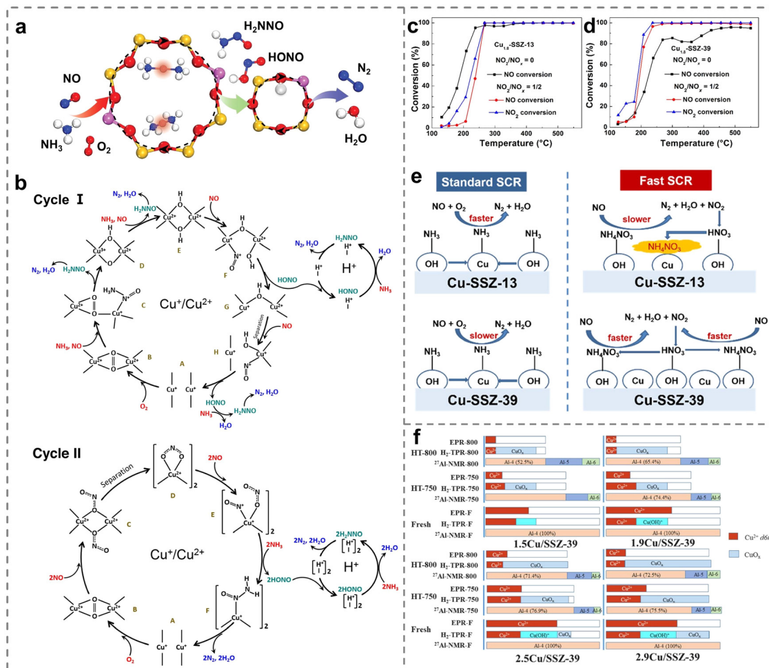
Fig. 4 (a) The reaction route in the multisite fashion for \text{NH}_3\text{-SCR} over \text{Cu-CHA} . (b) Two possible reaction mechanisms of \text{NH}_3\text{-SCR} . Copied with permission from ref. 77. Copyright 2020, American Chemical Society. (c) and (d) \text{NH}_3\text{-SCR} activity over (c) \text{Cu}_{1.8}\text{-SSZ-13} and (d) \text{Cu}_{1.8}\text{-SSZ-39} catalysts. Copied with permission from ref. 78. Copyright 2020, American Chemical Society. (e) The influences of \text{NO}_2 on \text{NH}_3\text{-SCR} processes on \text{Cu-SSZ-13} and \text{Cu-SSZ-39} . Copied with permission from ref. 79. Copyright 2021, Elsevier. (f) The contents of Al and Cu species quantified on \text{Cu/SSZ-39} zeolites. Copied with permission from ref. 79. Copyright 2021, Elsevier.
