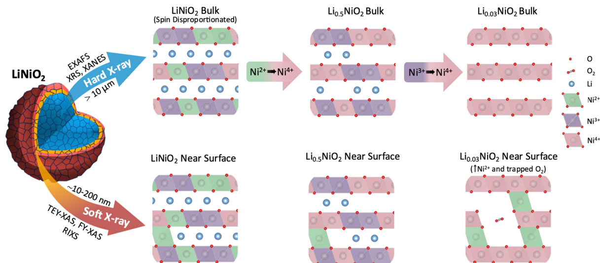
Fig. 6 Schematic representation of LiNiO 2 bulk charge compensation mechanism and surface degradation processes probed by different X-ray spectroscopy techniques. The differences in LiNiO 2 delithiation occurring at the surface and in the bulk, including the accommodation of trapped O 2 in pores formed near the surface by Ni 2+ species migrating to the Li layer. Continuous oxidation of Ni in bulk LiNiO 2 at high SoC is distinguished from the near surface degradation.
