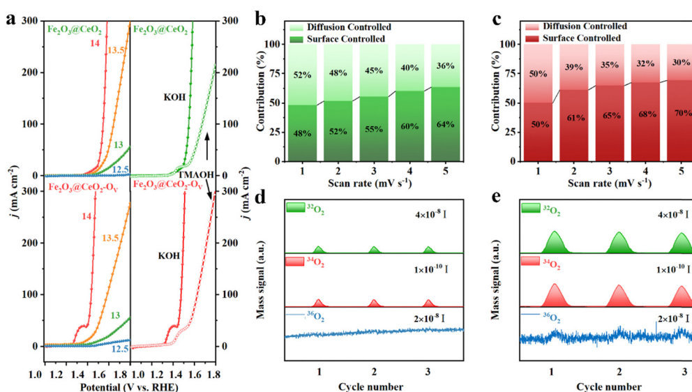
Fig. 5 OER performance of the prepared electrodes. (a) LSV curves of \text{Fe}_2\text{O}_3@/\text{CeO}_2\text{-O}_v and \text{Fe}_2\text{O}_3@/\text{CeO}_2 under different pH conditions (left) and in 1.0 M KOH or 1.0 M TMAOH, respectively (right). Contribution ratios of the capacitive and diffusion-controlled current densities vs. scan rates for (b) \text{Fe}_2\text{O}_3@/\text{CeO}_2 and (c) \text{Fe}_2\text{O}_3@/\text{CeO}_2\text{-O}_v . DEMS results by ^{18}\text{O} -isotopic labeling experiments for (d) \text{Fe}_2\text{O}_3@/\text{CeO}_2 and (e) \text{Fe}_2\text{O}_3@/\text{CeO}_2\text{-O}_v .
