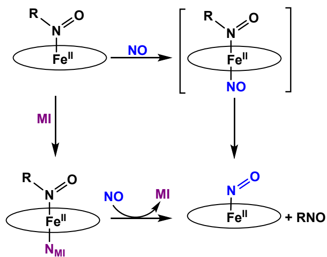
Scheme 3. Summary of the reactivity observed for five- and six-coordinate ferrous heme-RNO (R = IPr, PhNO) complexes with the TPP 2- ligand with NO.
