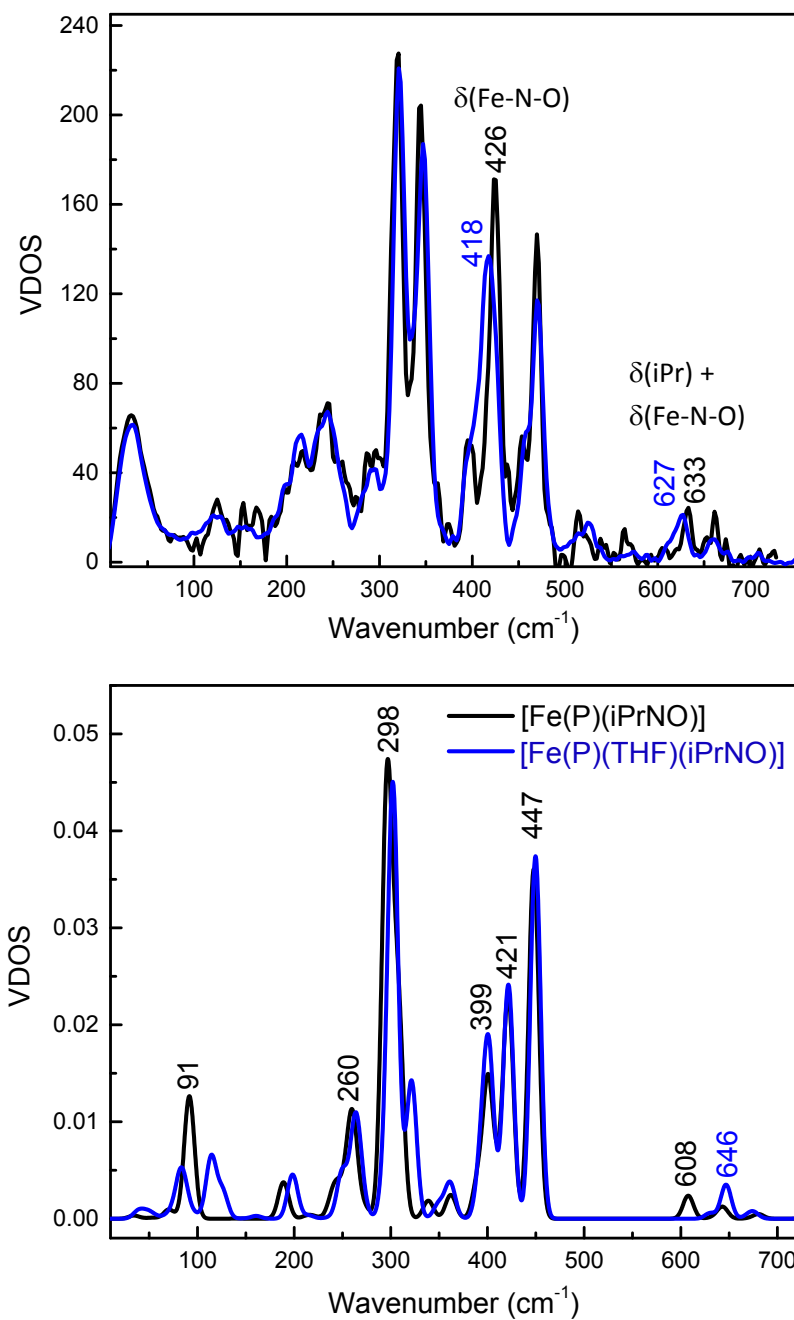
Figure 7. Top: NRVS-derived vibrational density of states (VDOS) for [\text{}^{57}\text{Fe}(\text{TPP})(\text{THF})(\text{iPrNO})] (black) and the ^{15}\text{N} -labeled iPrNO complex (blue). Bottom: BP86/TZVP calculated NRVS VDOS for [\text{Fe}(\text{P})(\text{iPrNO})] (black; \text{P}^{2-} = porphine dianion) and [\text{Fe}(\text{P})(\text{THF})(\text{iPrNO})] (blue).
