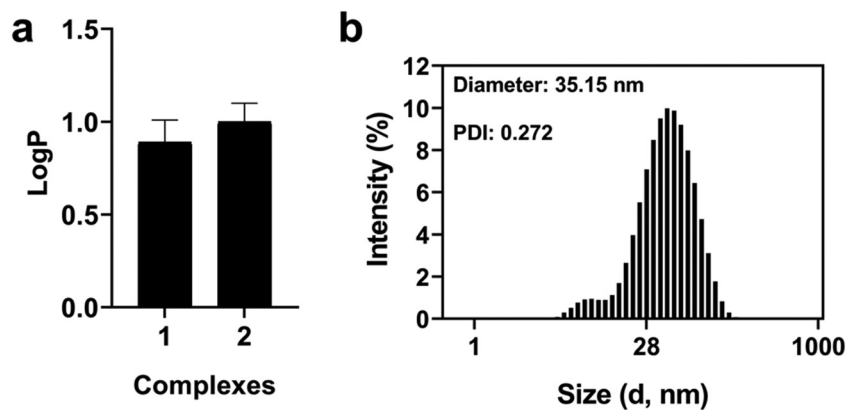
Fig. 4 Solubility and aggregation of Ru(II) complexes 1 and 2a/2b. (a) Partition coefficient between n -octanol/PBS and (b) size distribution by the intensity (20 \mu M) in PBS 10% FBS.
