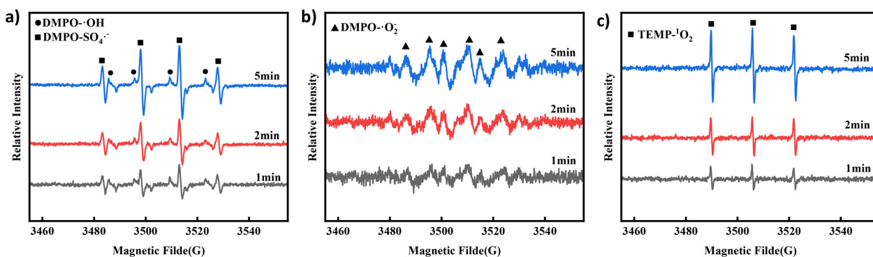
Fig. 4 EPR spectra of (a) DMPO· \cdot\text{OH} and DMPO· \text{SO}_4^{\cdot-} , (b) DMPO· \text{O}_2^{\cdot-} and (c) TEMP· ^1\text{O}_2 at different reaction times in the Co NP-PBC/PMS/TCH system.
