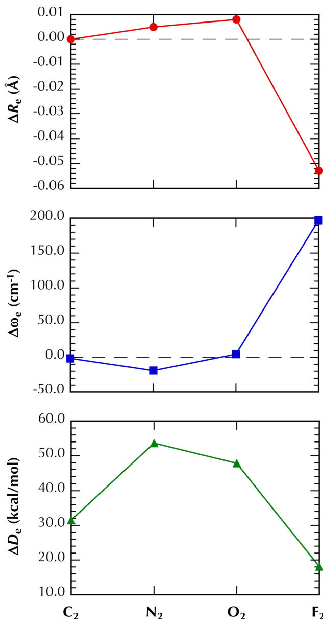
Fig. 1 Changes in the spectroscopic constants of \text{C}_2 - \text{F}_2 resulting from inclusion of dynamical electron correlation, e.g., \Delta R_e = R_e(\text{vCASI}) - R_e(\text{SCGVb}) .
