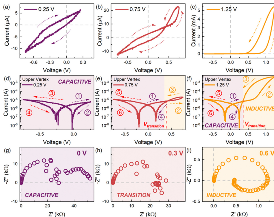
Fig. 7 A. Characteristic current–voltage ( I – V ) response in the linear scale of the halide perovskite memristor device FTO/poly(3,4-ethylenedioxythiophene) polystyrene sulfonate (PEDOT:PSS)/CH 3 NH 3 PbBr 3 /Au with varying upper vertex voltages of (a) 0.25 V, (b) 0.75 V, and (c), 1.25 V, with the arrows indicating the scan direction. The corresponding I – V response in the semi-log scale for upper vertex voltages of (d) 0.25 V, (e) 0.75, and (f) 1.25 V with the arrows and numbers indicating the scan direction and sequence, respectively. Voltage-dependent impedance spectral evolution measured at (g) 0 V, (h) 0.3 V, and (i) 0.6 V exhibiting a transition from a low frequency capacitive response at low applied voltages to a low frequency inductive response at high applied voltages. Figure courtesy of Cedric Gonzales. Reproduced by permission from J. Bisquert, Inductive and capacitive hysteresis of current–voltage curves. A unified structural dynamics in solar energy devices, memristors, ionic transistors and bioelectronics., PRX Energy , 2023, 3 , 011001, 35 licensed under a Creative Commons Attribution (CC BY 4.0) license.
