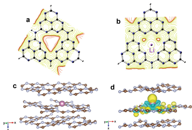
Fig. 6 Equipotential curve distribution on g-C 3 N 4 (a) and Li doped g-C 3 N 4 (b). Reproduced with permission from ref. 78. Copyright 2020, Elsevier. The optimized structure of g-C 3 N 4 with interlayer In doping (c); differential charge density of In doped g-C 3 N 4 (d), where the yellow and green isosurfaces represent the gain and loss of electrons, respectively. Reproduced with permission from ref. 80. Copyright 2021, Royal Society of Chemistry.
