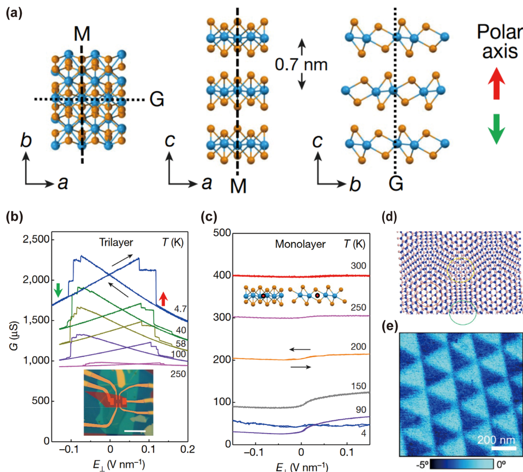
Fig. 10 (a) Top view, side view and front view of the 1T'-WTe 2 homotrilaier, M represents the mirror plane; G is the sliding plane; red arrow up and green arrow down are polar c-axes. W atoms are in blue; Te atoms are in orange. (b) Conductance G of the undoped trilayer device as E_{\perp} is swept up and down (black arrows). The plots show bi-stability associated with electric polarization up (red arrow) or down (green arrow), at temperatures from 4 K to 300 K (as labelled). Inset is the optical image of a representative double-gated device. (c) Similar measurements on a monolayer 1T'-WTe 2 device (M1), showing no bistability. 173 Reprinted with permission from ref. 173. Copyright 2018, Macmillan Publishers Ltd, part of Springer Nature. (d) Schematic diagram of twisted bilayer h-BN forming moiré superlattice ferroelectricity. 25 Reprinted with permission from ref. 25. Copyright 2017, American Chemical Society. (e) Twisted h-BN ferroelectric domain image with a triangular period. 175 Reprinted with permission from ref. 175. Copyright 2021, The Authors, published by Springer Nature.
