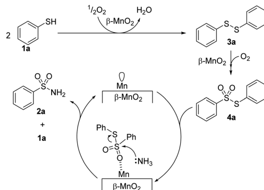
Fig. 9 Proposed reaction mechanism for the one-pot aerobic sulfonamidation of benzenethiol ( 1a ) to benzenesulfonamide ( 2a ) with \beta\text{-MnO}_2 -1. (Reproduced from ref. 59 with permission from Royal Society of Chemistry).
