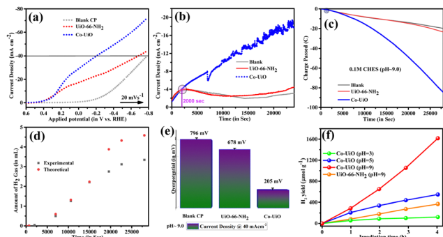
Fig. 2 (a) Comparative linear sweep voltammetry (LSV) data recorded for the catalyst-modified electrodes at pH \sim 9.0. LSV was recorded after CV stabilised at 20 \text{mV s}^{-1} scan rate; data were recorded at room temperature using 0.1 M CHES buffer. The active surface area of the CP-modified electrode was 0.25 \text{ cm}^2 . (b) Chronoamperometric current passed with time during the fixed potential electrolysis at -0.490 \text{ V} in a 0.1 M CHES buffer (pH \sim 9.0) (the purple circle indicated the boost in HER activity). (c) Chronocoulometric charge passed during the fixed potential electrolysis at -0.472 \text{ V} (the purple circle indicated the boost in HER activity). [In Figure a, b, c; Gray trace: blank CP, red trace: UiO-66-NH 2 modified CP, and blue trace: Co-UiO modified CP.] (d) The experimentally (black trace) and theoretically (red trace) measured volume of H 2 gas during the bulk electrolysis at pH \sim 9.0. (e) Comparative bar diagram for the overpotential requirement to attain 40 \text{ mA cm}^{-2} current density during the LSV experiment performed at pH \sim 9.0; and (f) time course of the photocatalytic H 2 production curves.
