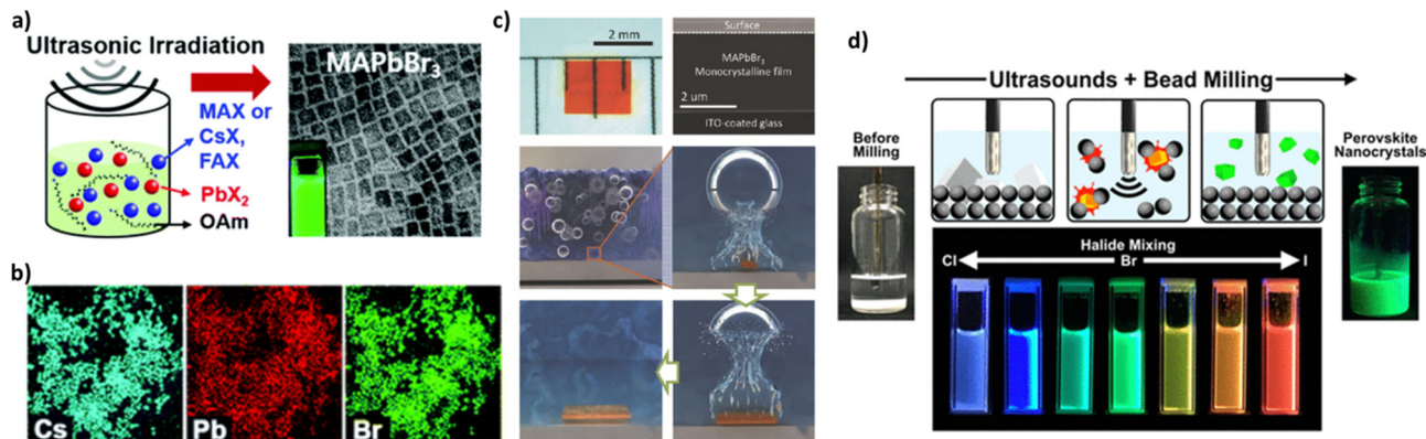
Fig. 13 (a) Ultrasound-induced synthesis of APbX_3 perovskite nanocrystals with a wide range of compositions, where A = CH_3NH_3 , Cs, or HN=CHNH_3 (formamidinium), and X = Cl, Br, \text{ or } I . (b) EDX maps showing homogeneous distributions of Cs, Pb, and Br in CsPbBr_3 NCs. Adapted with permission from ref. 186. (c) Optical image of the monocrystalline film (left). Cross-sectional SEM image of a freshly cut monocrystalline film (right). Illustrations of the CTAC mechanism on a microscopic scale. Adapted with permission from ref. 187. (d) Schematic illustration of the ultrasound-assisted bead milling (top) and photograph under a UV lamp of the colloidal halide-mixed perovskite nanocrystals. Adapted with permission from ref. 189.
