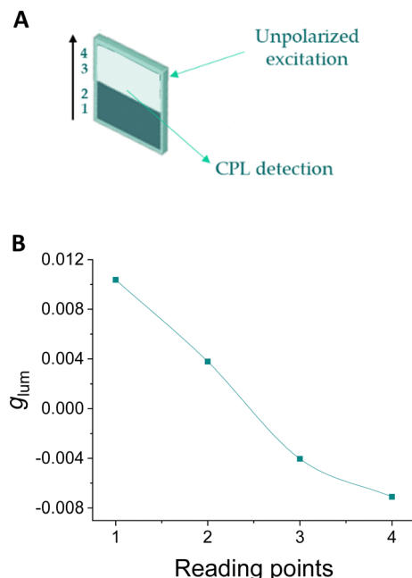
Fig. 10 (A) Method used for reading barcodes at 4 points, from (S,S,P)- 1 to (R,R,M)- 1 . (B) Reading of a barcode with two bands of 32 layers of (S,S,P)- 1 to (R,R,M)- 1 . Average signal of a small wavelength range. See Fig. S28 (ESI†) for raw data.
