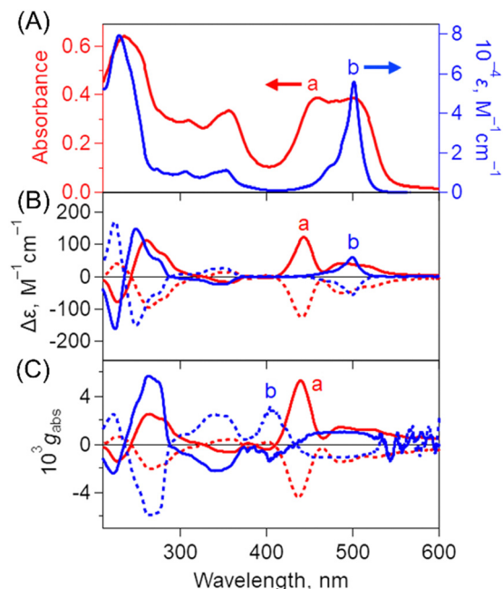
Fig. 4 (A) Absorption spectra of (a) (0Ph-B-BODIPY) m in H 2 O/THF = 99/1 ( v/v ). [0Ph-B-BODIPY] = 30 \mu M and (b) 0Ph-B-BODIPY in THF. (B) CD spectra of (a) (0Ph-B-BODIPY) m in H 2 O/THF = 99/1 ( v/v ). [0Ph-B-BODIPY] = 30 \mu M and (b) 0Ph-B-BODIPY in THF. Solid and dotted lines correspond to S and R forms, respectively. (C) Dissymmetry factor g_{\text{abs}} profiles of (a) (0Ph-B-BODIPY) m in H 2 O/THF = 99/1 ( v/v ). [0Ph-B-BODIPY] = 30 \mu M in H 2 O/THF and (b) 0Ph-B-BODIPY in THF. Solid and dotted lines correspond to S and R forms, respectively.
