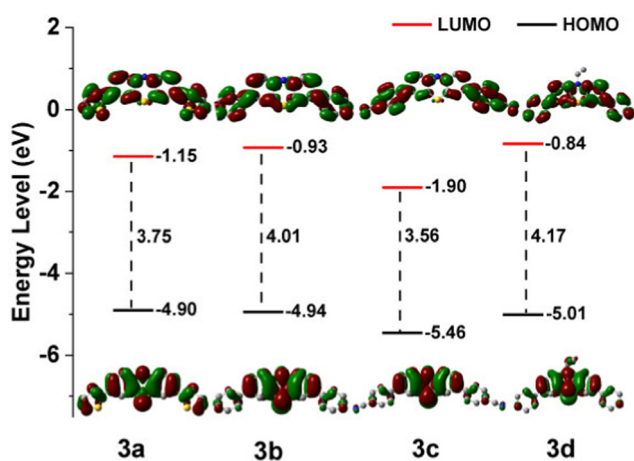
Fig. 2 Experimental orbital energy levels and HOMO/LUMO orbital plots of 3a , 3b , 3c and 3d .
