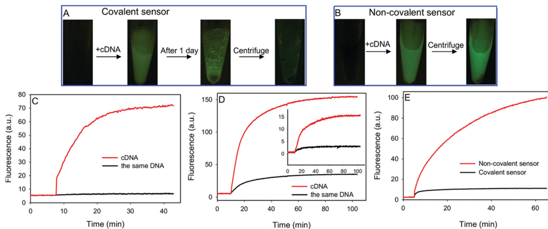
Fig. 8 Photographs of fluorescence associated with GO sensors prepared using covalent (A) and non-covalent (B) DNA probes after washing with cDNA and centrifugation. Fluorescent response of the covalently (C) and non-covalently (D) prepared GO sensors after the addition of cDNA and same-DNA (probe DNA lacking a fluorescent label). The inset of panel (D) is with 10-fold less probe DNA. (E) Fluorescent response of the covalently and non-covalently prepared GO sensors in the presence of 0.5% BSA. Reproduced from ref. 50 with permission from the American Chemical Society.
