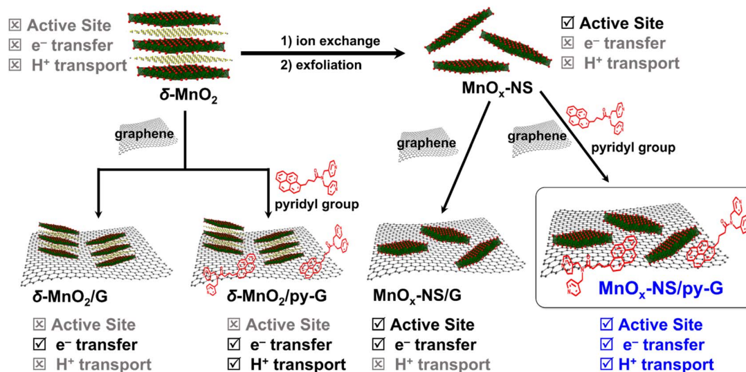
Scheme 2 Schematic illustration of the synthetic procedure of MnO x -NS/G, MnO x -NS/py-G, δ-MnO 2 /G, and δ-MnO 2 /py-G.
